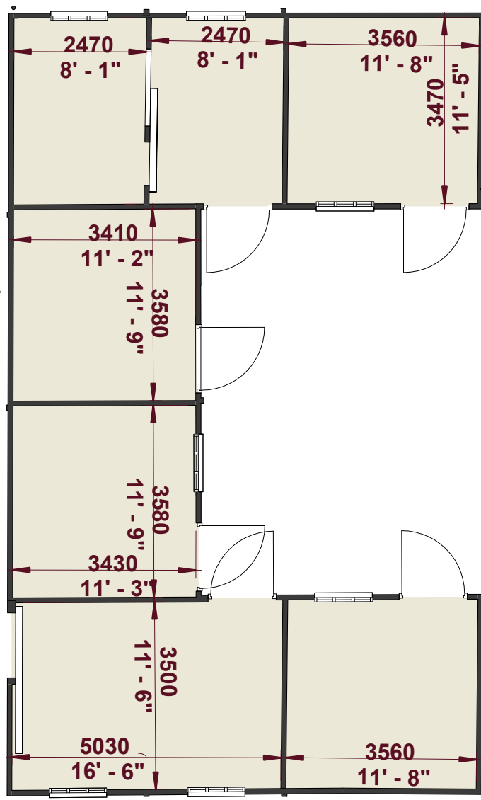
Stable - Existing Ground Floor 1 : 100
